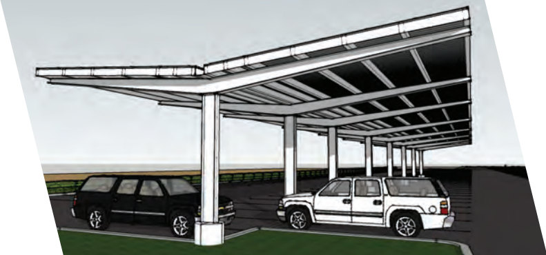
Typical Carport 6 Y with Deck and Gutter
